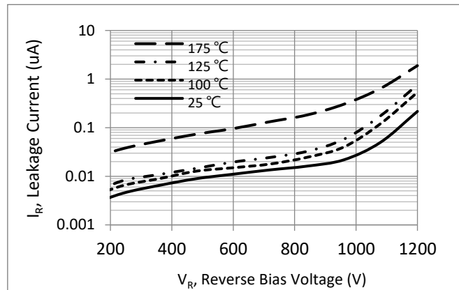
Fig.2 Reverse Characteristics
