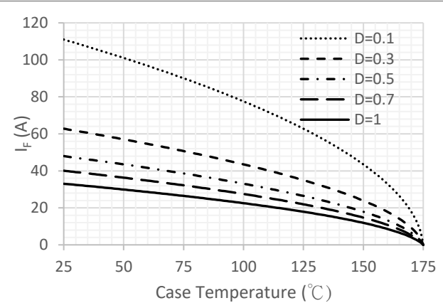
Fig.4 Maximum Forward Current
