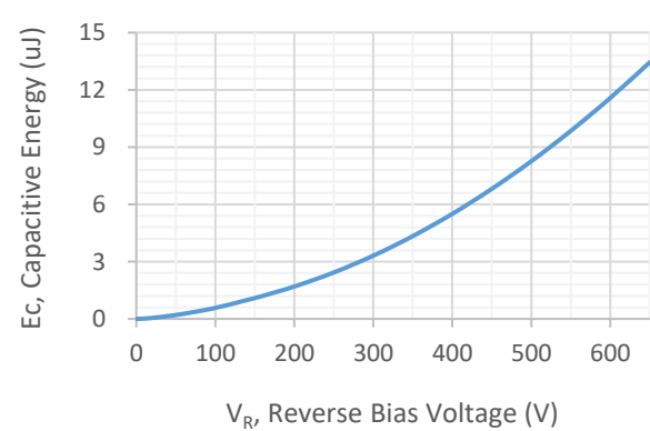
Fig.6 Capacitance Stored Energy
