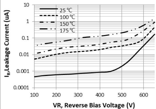
Fig.2 Reverse Characteristics
