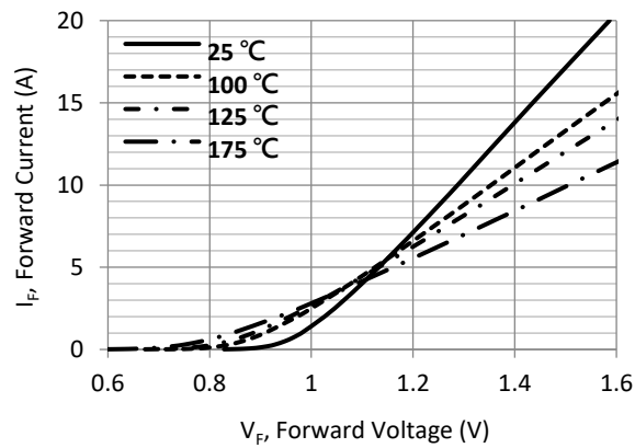
Fig.1 Forward Characteristics
