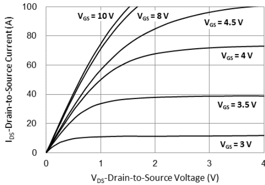
Fig.1 On-Region Characteristics
