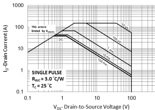
Fig.11 Maximum Safe Operating Area
