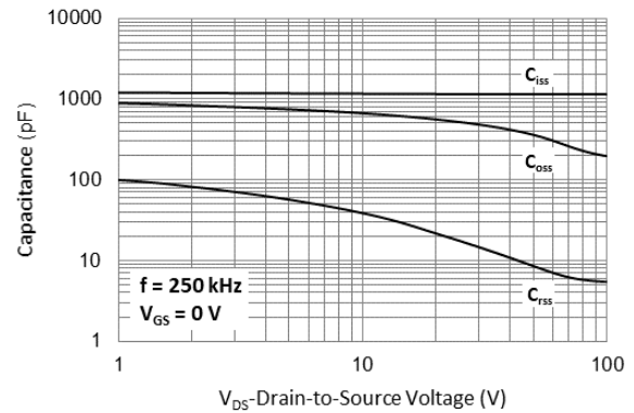
Fig.10 Capacitance vs. Drain-Source Voltage
