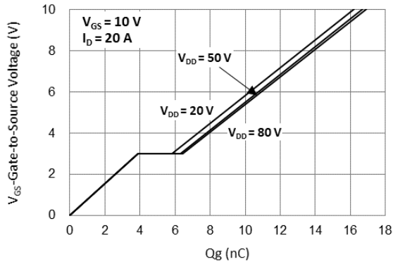
Fig.7 Gate-Charge Characteristics
