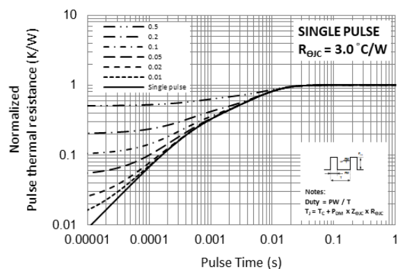
Fig.12 Normalized Transient Thermal Impedance
