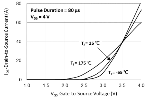
Fig.2 Transfer Characteristics
