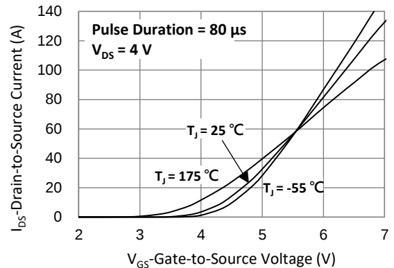
Fig.2 Transfer Characteristics
