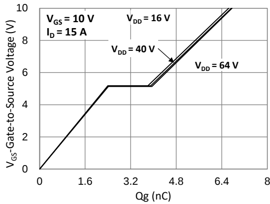
Fig.7 Gate-Charge Characteristics
