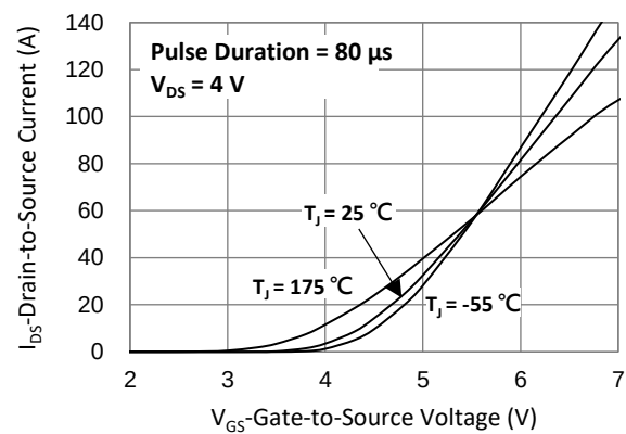
Fig.2 Transfer Characteristics
