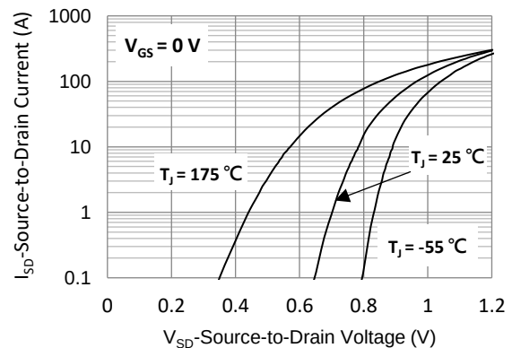
Fig.6 Source-Drain Diode Forward Voltage
