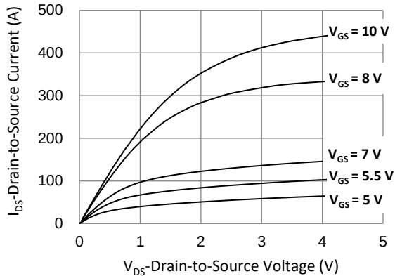
Fig.1 On-Region Characteristics
