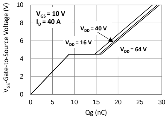
Fig.7 Gate-Charge Characteristics
