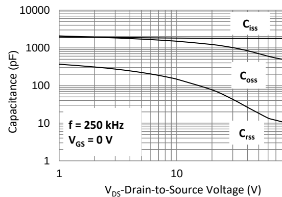
Fig.10 Capacitance vs. Drain-Source Voltage
