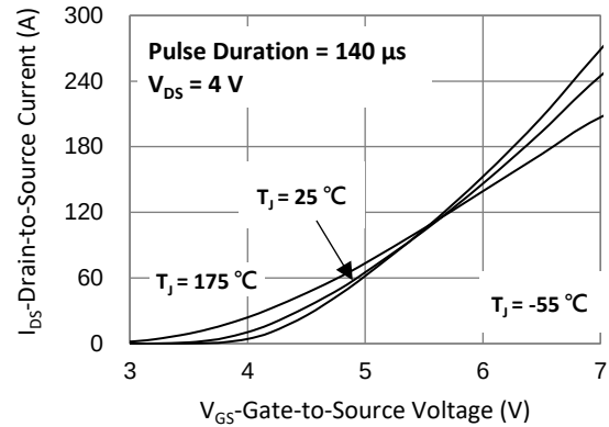
Fig.2 Transfer Characteristics
