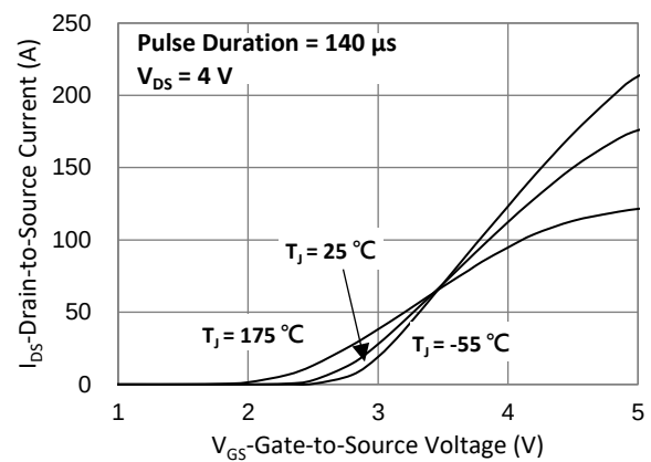
Fig.2 Transfer Characteristics
