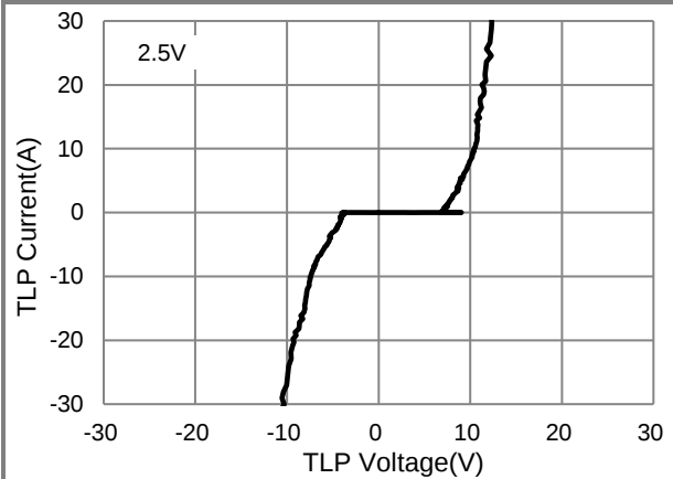
Fig.4 TLP Measurement
