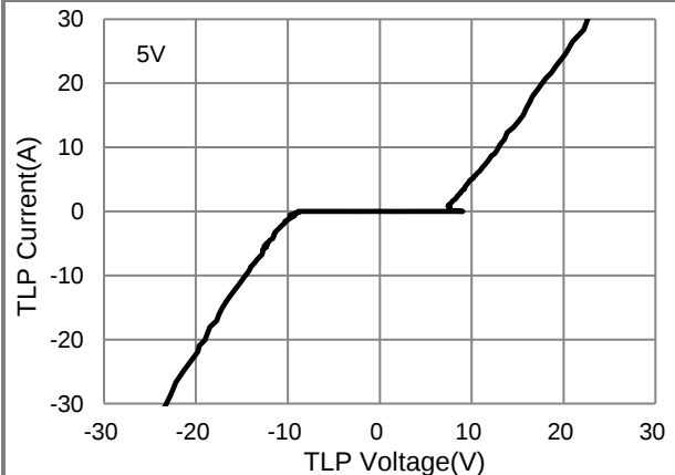
Fig.6 TLP Measurement
