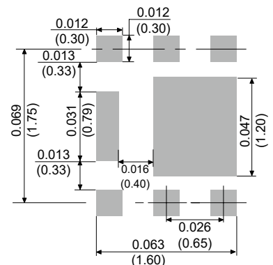
DFN2020B-6L
