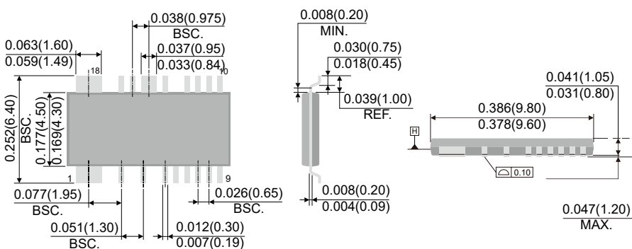
TSSOP-18
