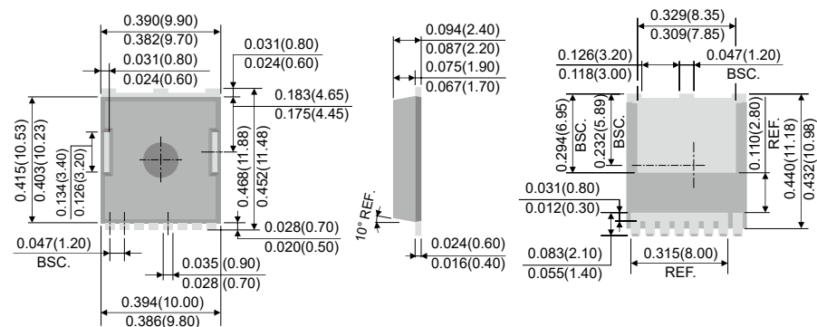
TOLL
