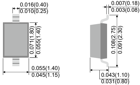
SOD-123HE
