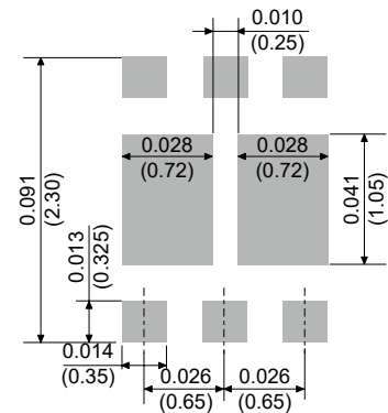
DFN2020-6L
