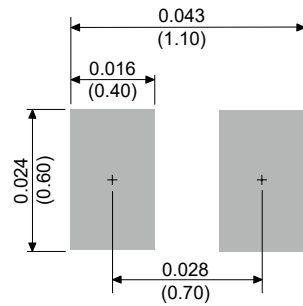
DFN1006-2L
