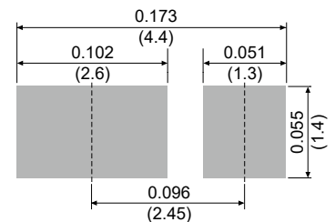
SOD-123HE
