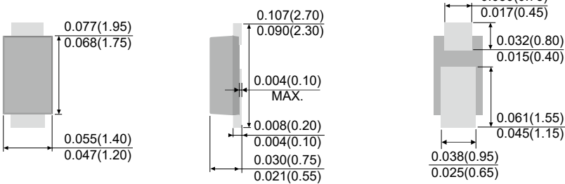
SOD-323
