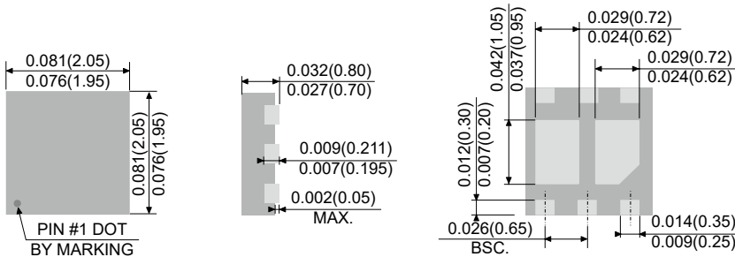
DFN2020-6L
