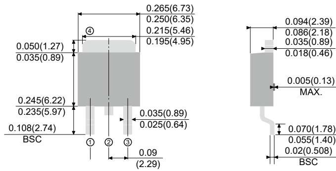
TO-252AA-2LD
