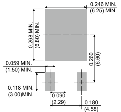
TO-252AA-2LD
