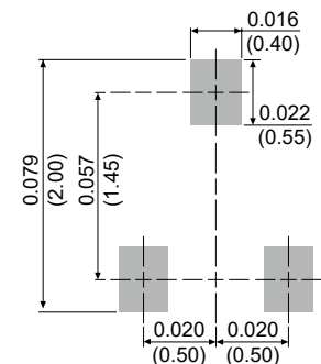
SC-89
