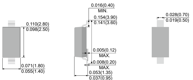
SOD-123
