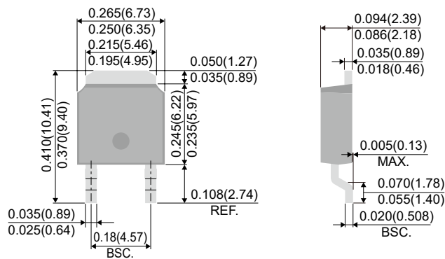
TO-252AA-2LD
