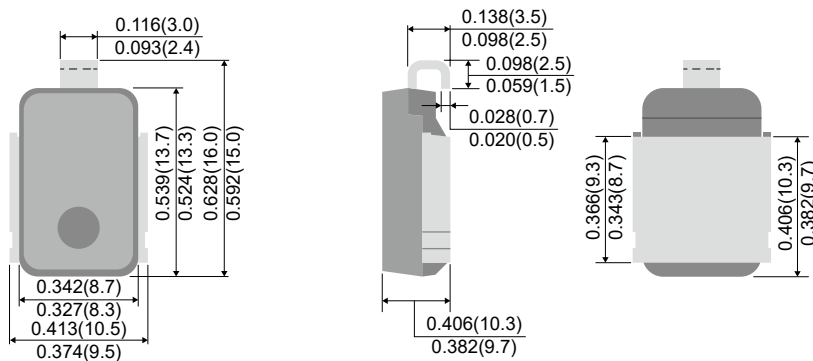
DO-218AB
