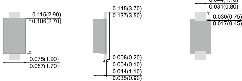
SOD-123
