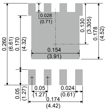
DFN5060S-8L
