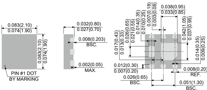
DFN2020B-6L
