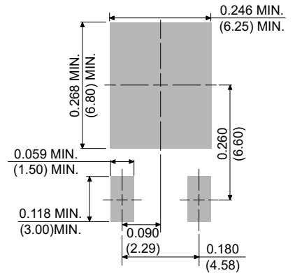
DO-218AB
