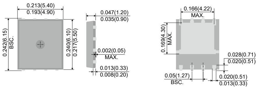
DFN5060X-8L
