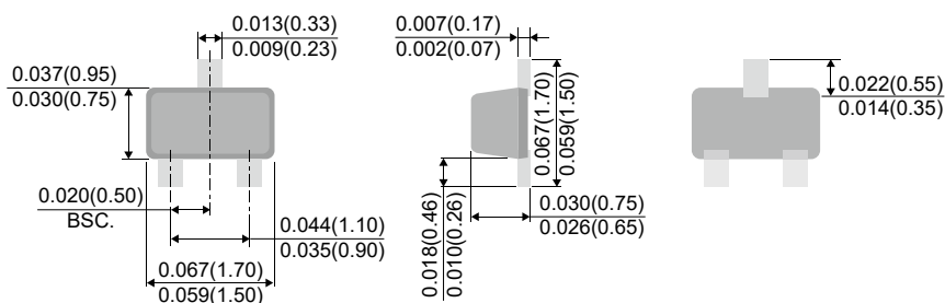
SC-89
