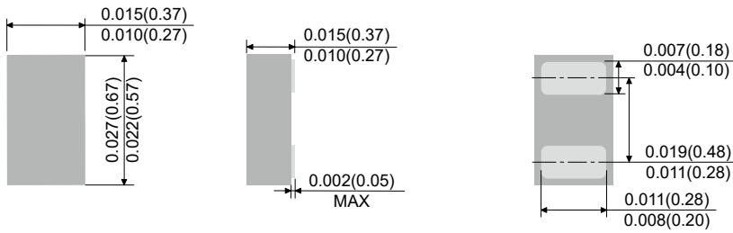
DFN0603-2L
