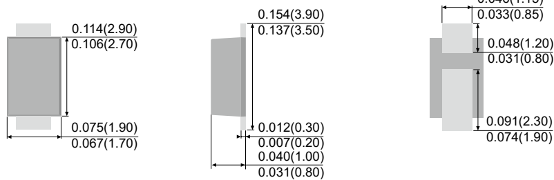
SOD-123FL
