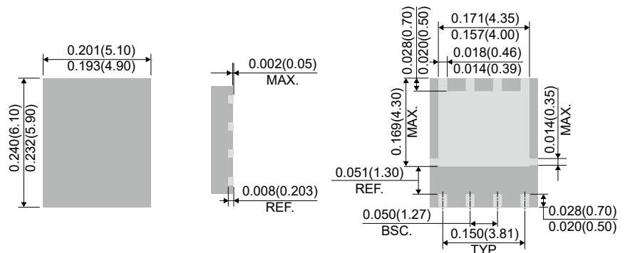
DFN5060S-8L
