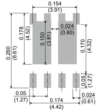
DFN5060X-8L
